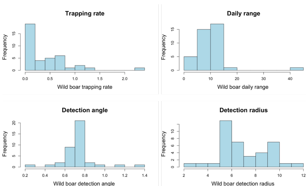
Figure 6. Distributions of the REM parameters estimated from Wild Boar CT sequences in 39 EOW study sites in 2023.
