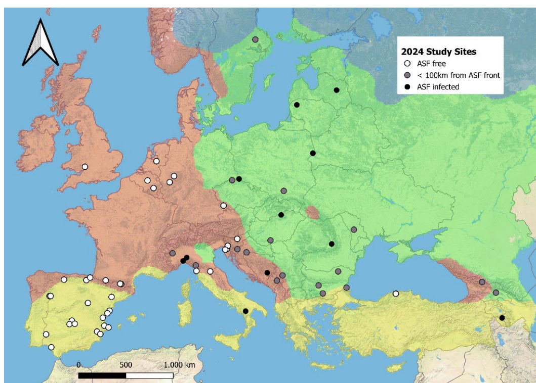
Figure 19. Distribution of the EOW sites with respect to their location in ASF-infected areas, in proximity of ASF (<100km from an infected area) or far from ASF (>100km from an infected area). Colours represent bioregions: Southern (yellow), Western (red), Eastern (green) and Northern (blue).
