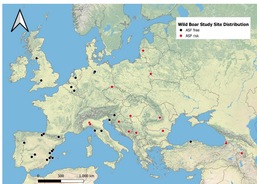
Figure 5. - EOW study sites, where wild boar density was estimated through the REM method in 2023. Sites in ASF-infected areas or nearby ( <100\text{km} ) are in red.
